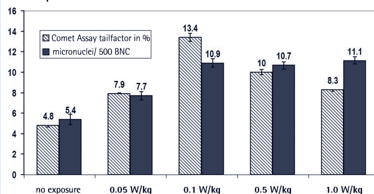
Dose-dependent increase in DNA strand breaks
