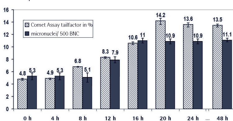
Time-dependent formation of DNA strand breaks
